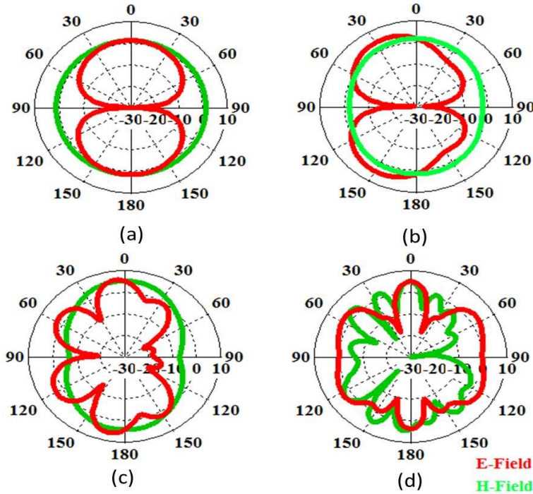
Figure 4. 10 Simulated radiation patterns of the Sierpinski Gasket diamond at (a) 1 GHz, (b) 2.5 GHz, (c) 5.8GHz (d) 12.6 GHz.
