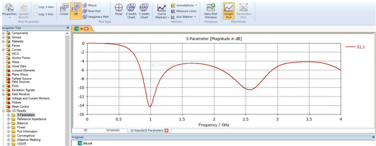
Figure 4.2 Simulated return loss curve for Initiator
