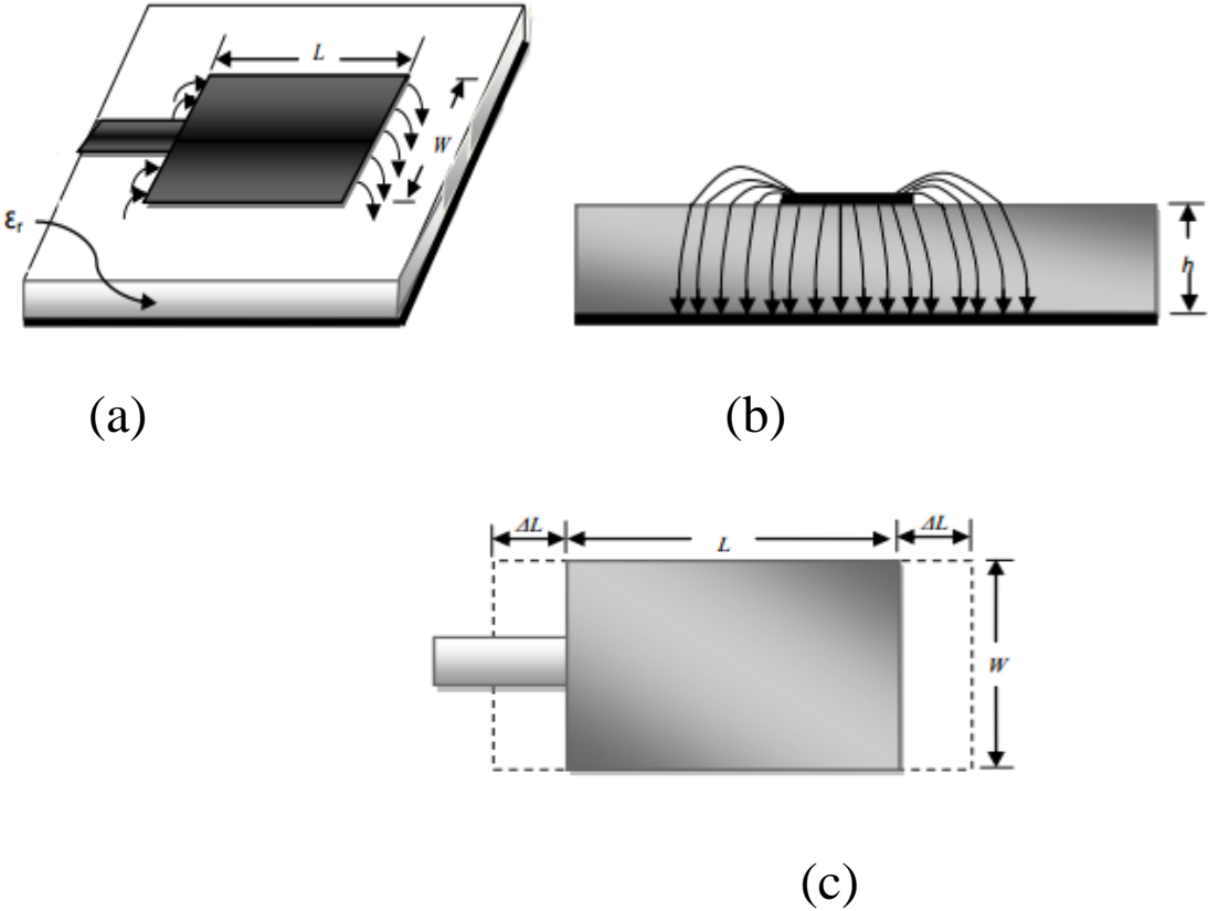
Figure 2. 1 Microstrip antenna (a) top view, (b) Electrical field lines,(c) Equivalent length
