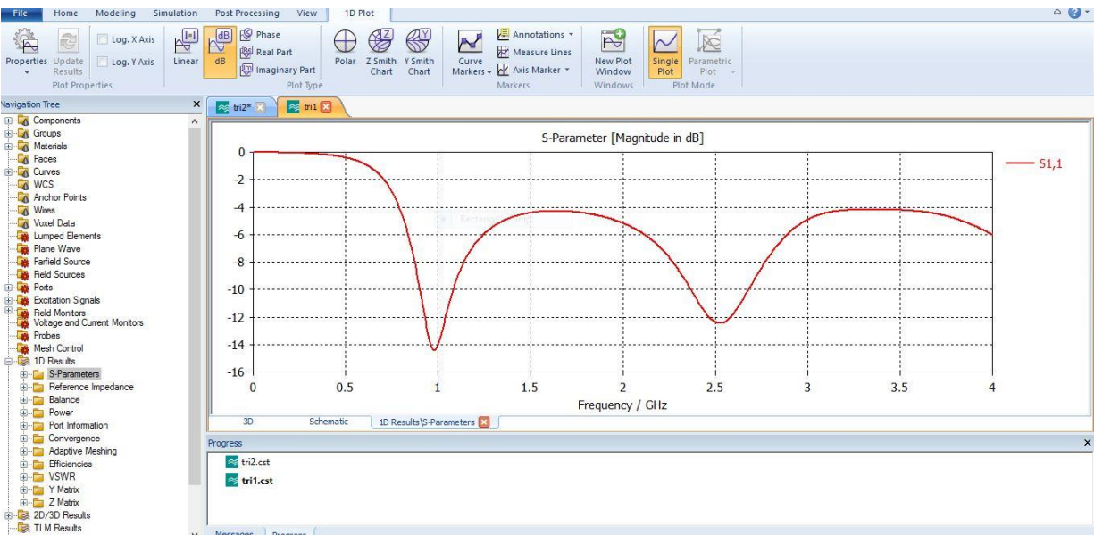
Figure 4. 4 Simulated return loss curve for First iterated Sierpinski Gasket Diamond antenna
