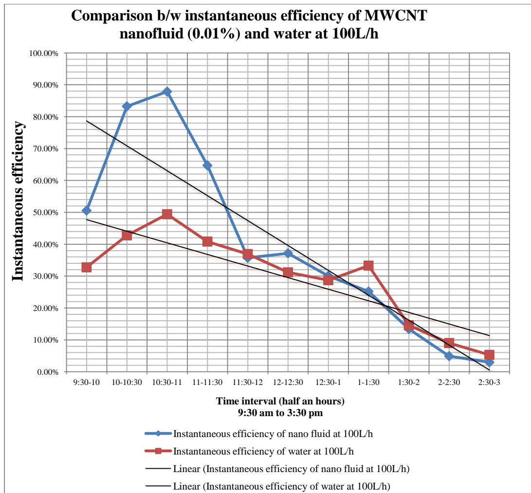
Figure 45: Experimental variations in instantaneous efficiency of water and nano fluid (0.01%) with change in day time at 100L/h
