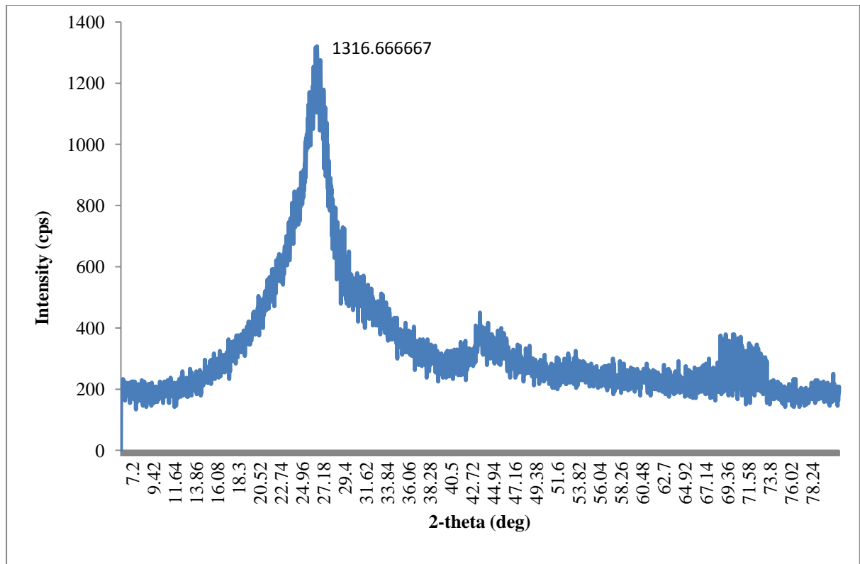
Figure 25: X-Ray Diffraction Graph for MWCNTs
