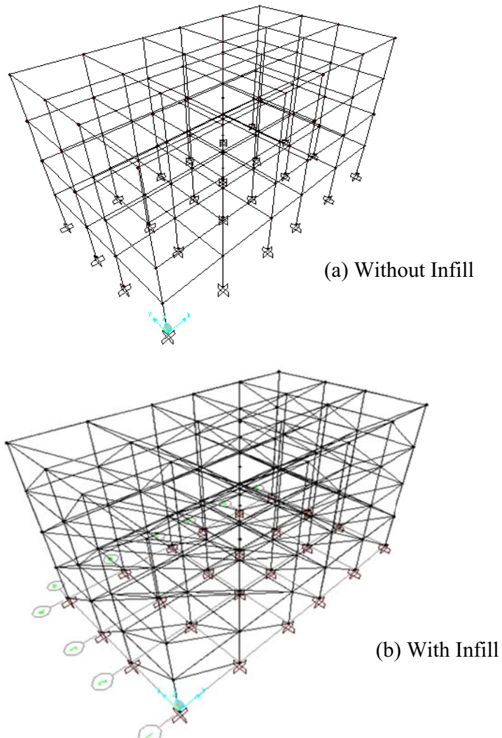
Fig. 3.3: 3D Computer model of building without and with considering infill stiffness respectively.
