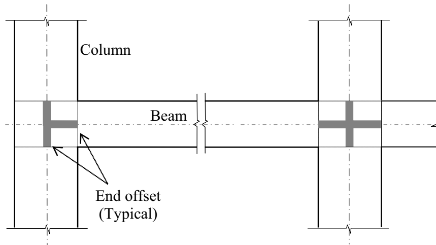
Fig. 3.2: Use of end offsets at beam-column joint
