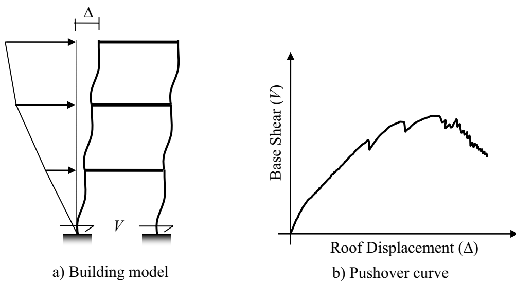
Fig. 5.1: Schematic representation of pushover analysis procedure
