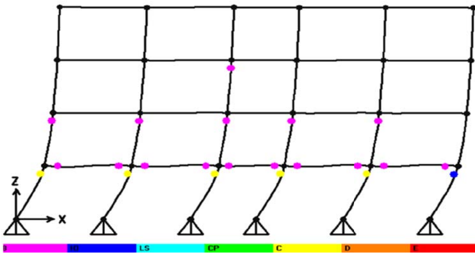
Fig. 5.4 (a): Distribution of plastic hinges for WI building model
