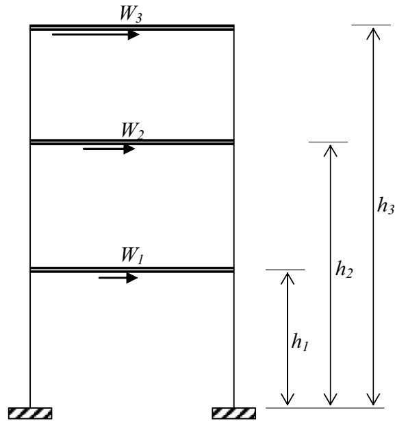
Fig. 4.2: Building model under seismic load
