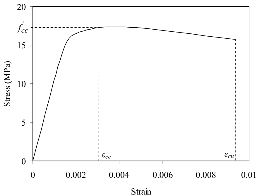
Fig. 3.5: Typical stress-strain curve for M-20 grade concrete (Panagiotakos and Fardis, 2001)
