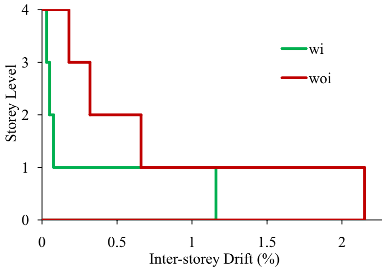
(a) for pinned-end building model
