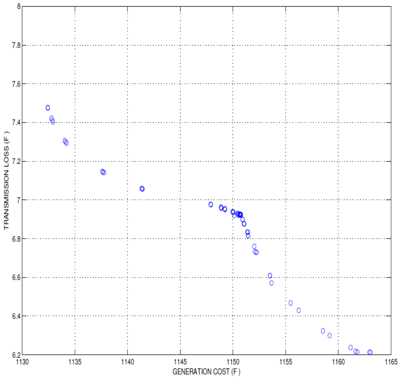
FIG-6.1 2D PLOT FOR F vs F OF IEEE-14 BUS SYSTEM
