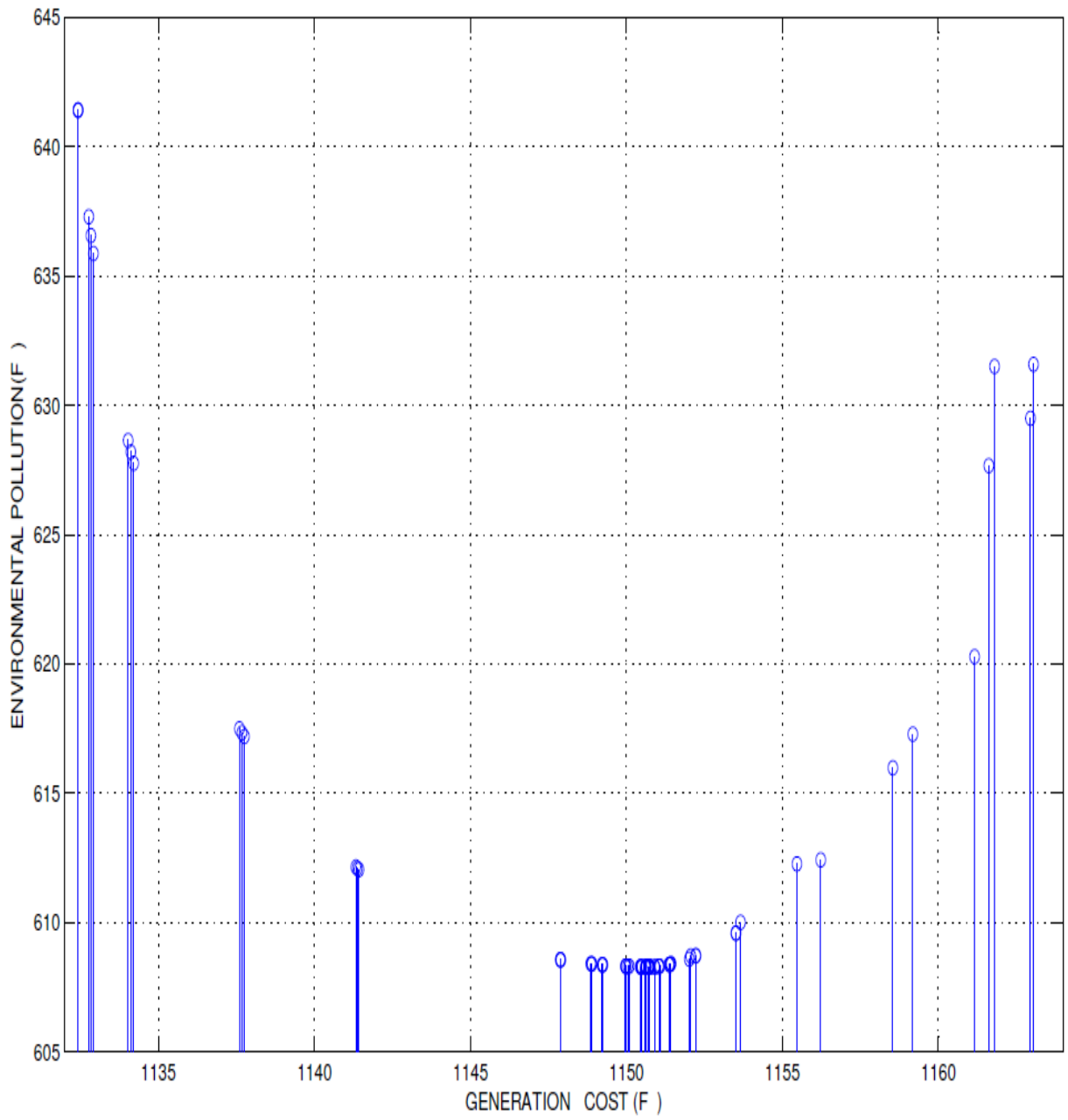
FIG-6.2 2D PLOT FOR F VS F OF IEEE-14 BUS SYSTEM
