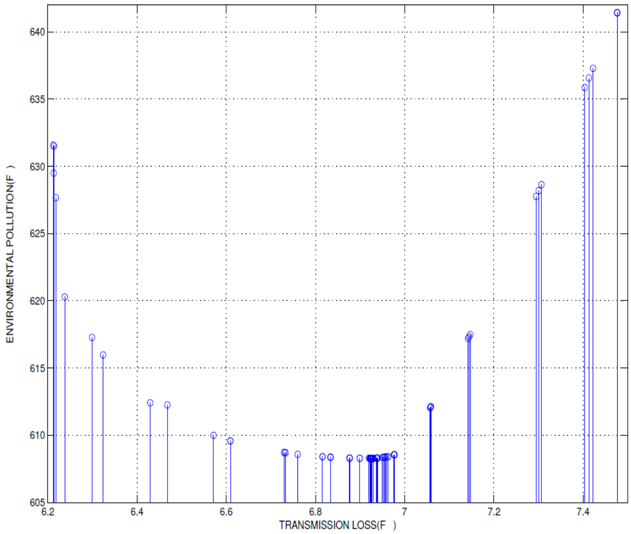
FIG-6.3 2D PLOT FOR F V/S F OF IEEE-14 BUS SYSTEM
