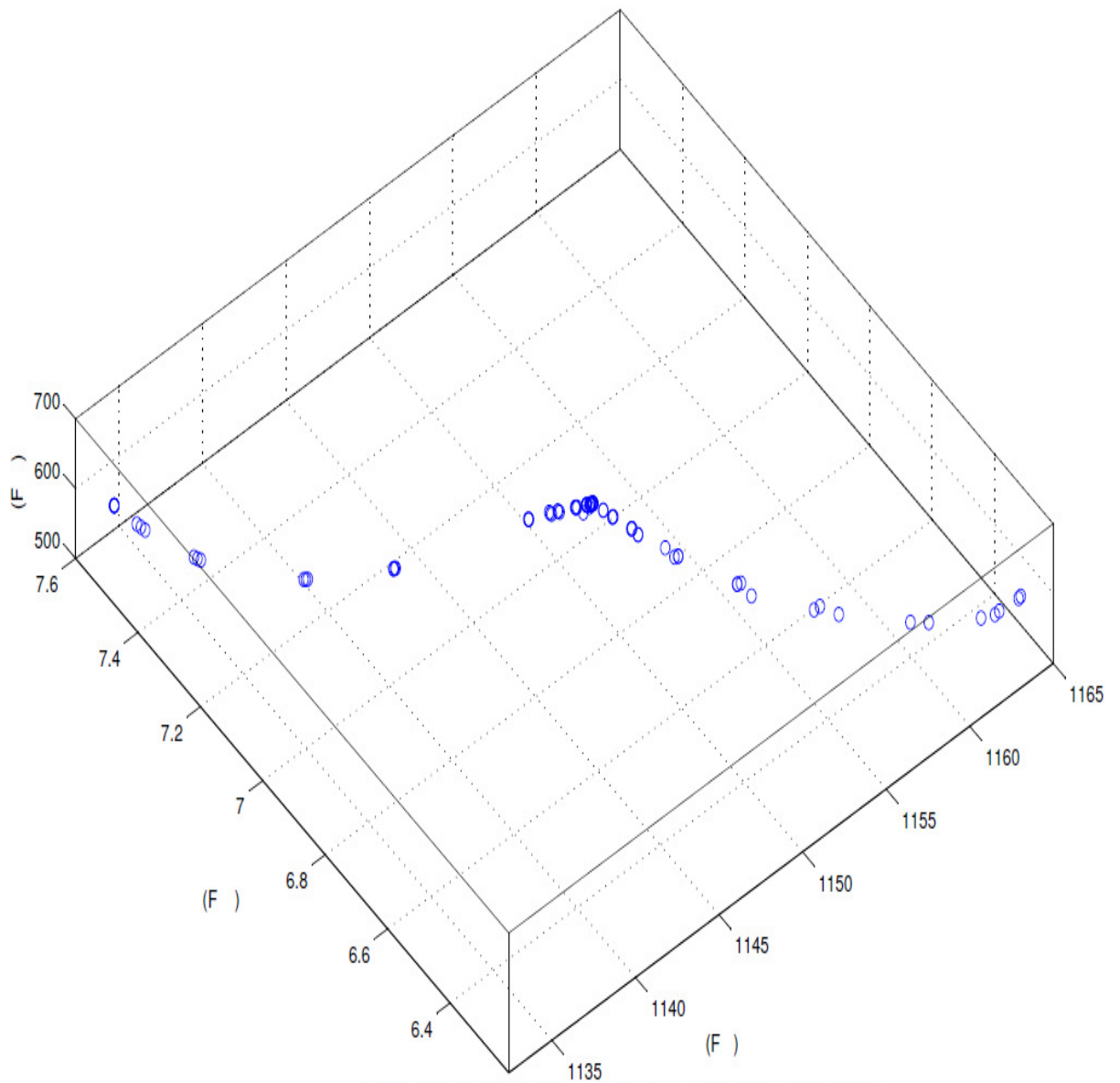
FIG-6.4 NONINFERIOR CURVE OF IEEE -14 BUS SYSTEM IN 3D SPACE
