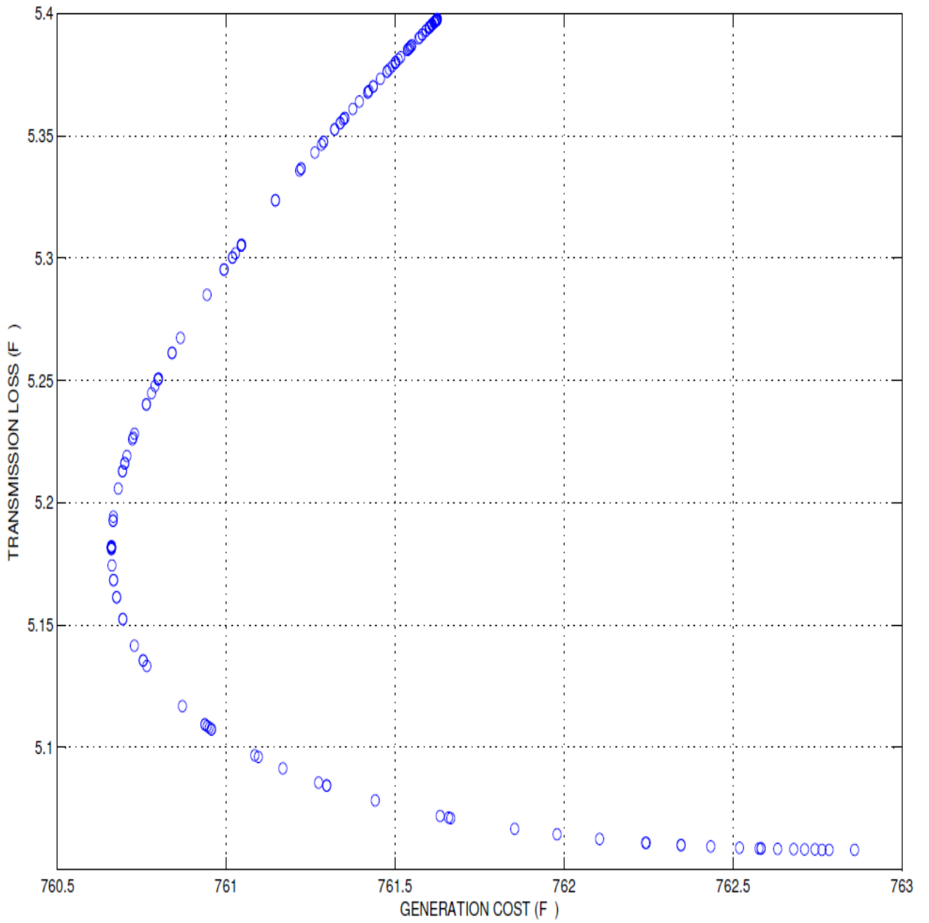
FIG-6.3 2D PLOT FOR F VS F OF IEEE-5 BUS SYSTEM
