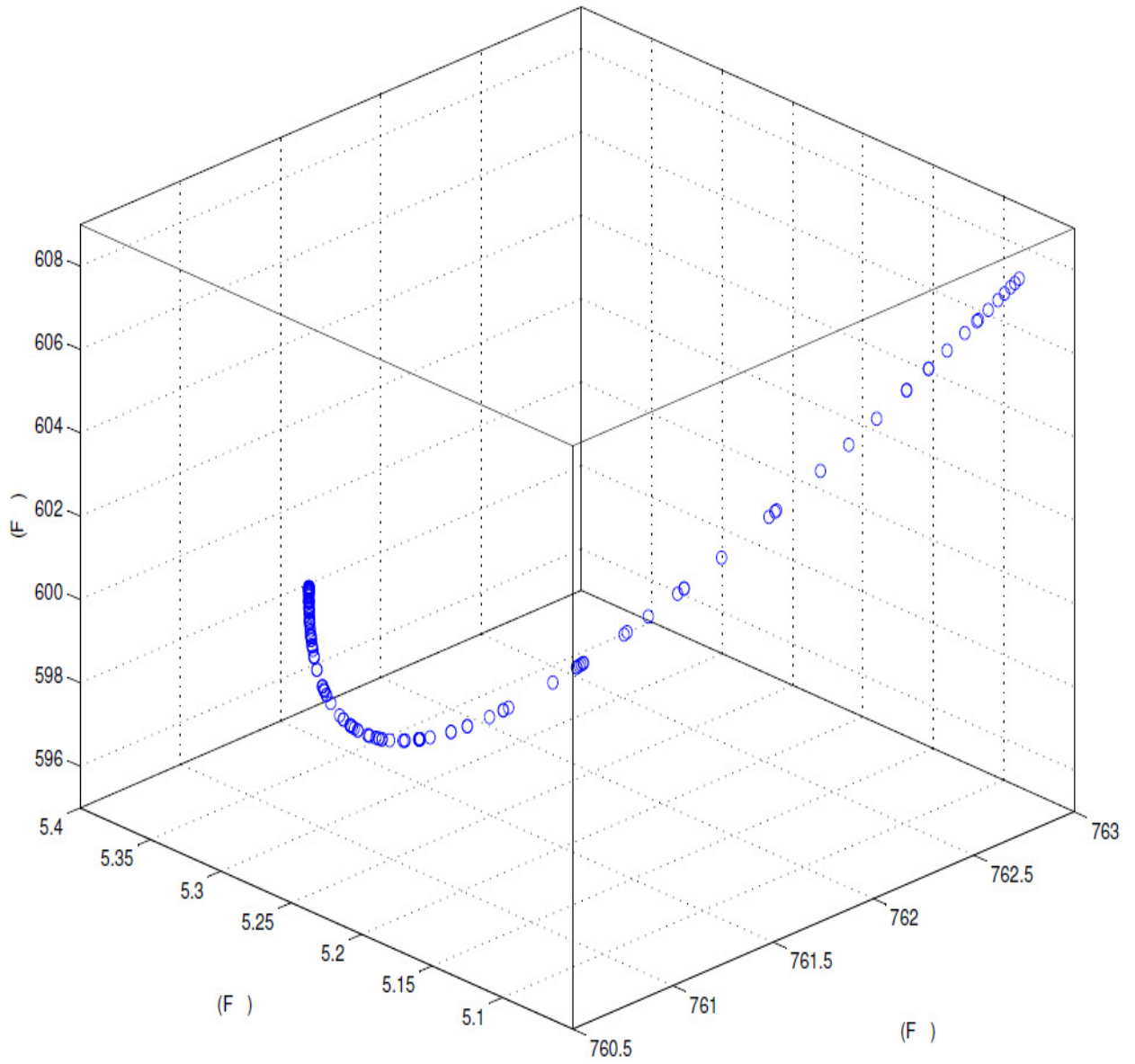
FIG-6.4 NONINFERIOR SET OF IEEE-5 BUS SYSTEM IN 3D SPACE
