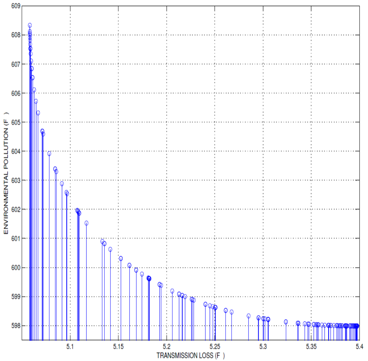
FIG-6.1 2D PLOT FOR F VS F OF IEEE-5 BUS SYSTEM
