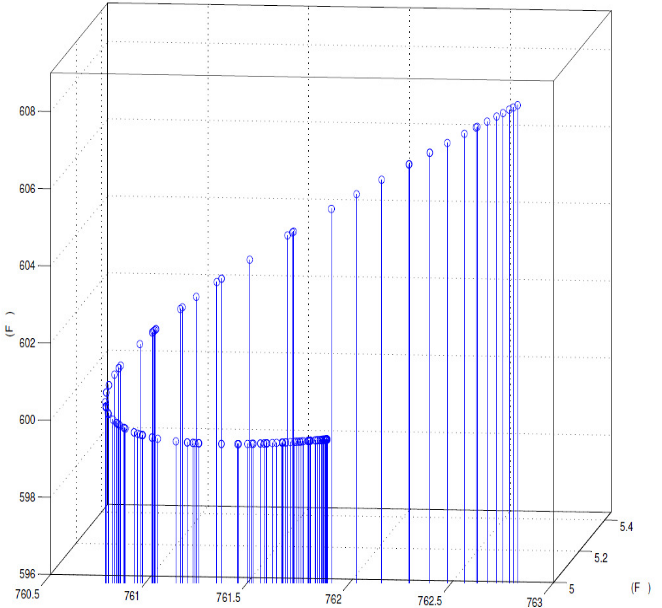
(F) FIG-6.5 NONINFERIOR SET OF IEEE-5 BUS SYSTEM IN 3D SPACE
