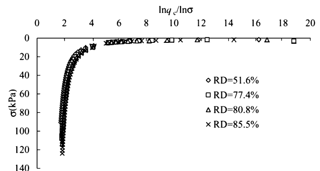
FIG. 4b— \ln q_c / \ln \sigma versus \sigma_{ov} for coal ash.
