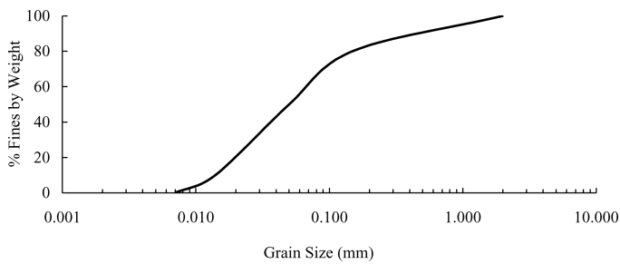
FIG. 2—Grain size distribution of coal ash.
